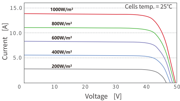
I-V Curves of PV Module
